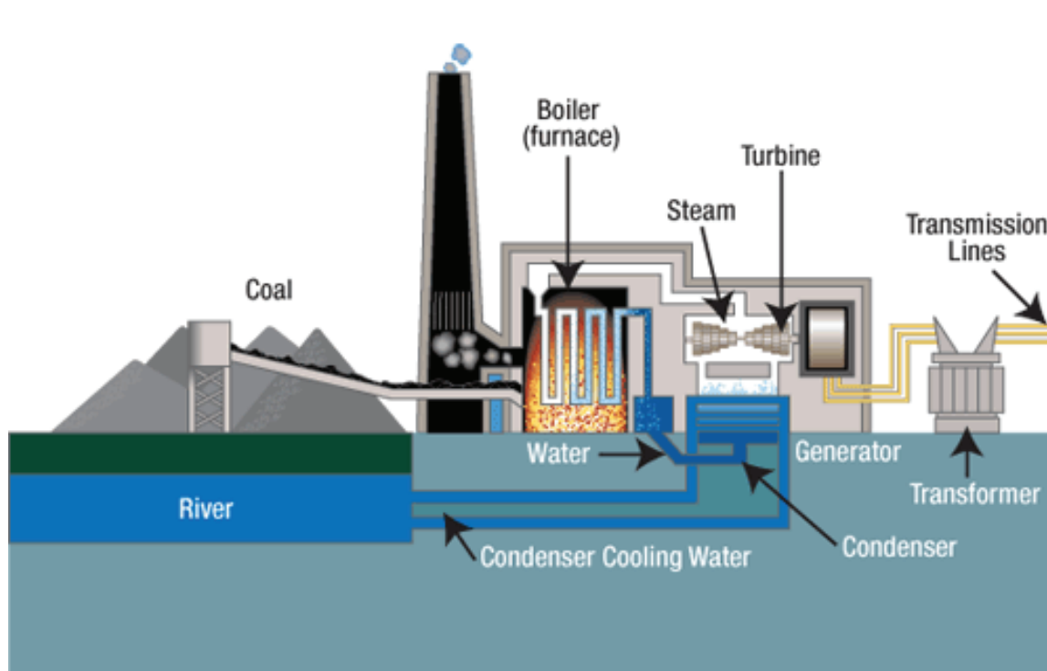
Coal-fired thermoelectric power generation plant.
